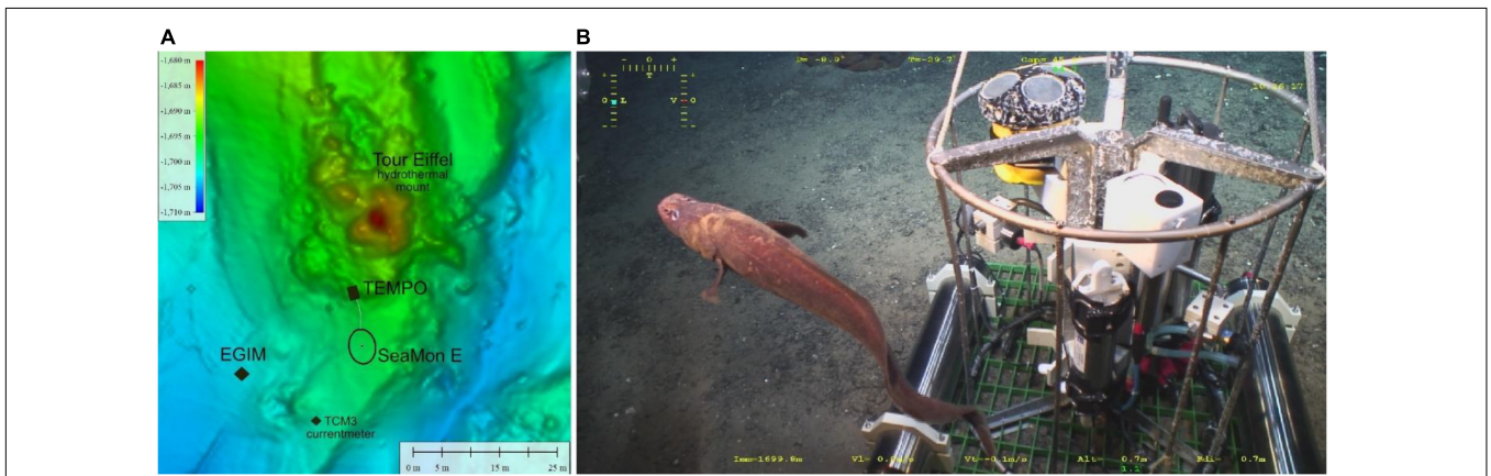
FIGURE 7 | (A) Map of the Tour Eiffel area at Lucky Strike (mid-Atlantic ridge) showing the location of the EGIM and the components of the EMSO-Azores observatory; (B) the EGIM.
