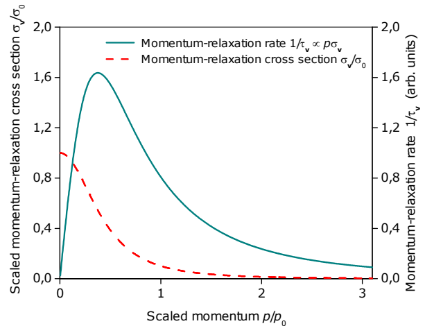
Fig. 5. The rate of momentum relaxation ( 1/\tau_v ) is plotted as a function of the scaled momentum together with the momentum-relaxation scattering cross section ( \sigma_v ) of the
