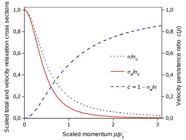
Fig. 4. The total scattering cross section ( \sigma ) and velocity-relaxation scattering cross section ( \sigma_v ) of the Yukawa potential v(\boldsymbol{\rho}) are plotted as functions of the momentum p . The momentum scale p_0 is \hbar/\rho_0 , where \rho_0 is the range of v(\boldsymbol{\rho}) . The cross sections have been scaled by the value \sigma_0 at a vanishing energy. Also shown is the ratio of velocity persistence c(p) , or average direction-cosine of the scattering angle (\mathbf{p}, \mathbf{p}') , as a function of p = p' .
