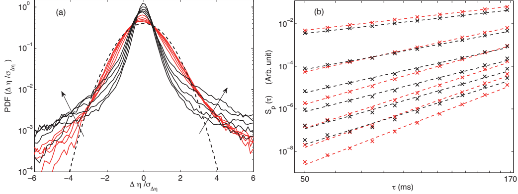
Figure 8: (a) Probability density functions of normalized increments \Delta\eta_t(\tau)/\sigma_{\Delta\eta_t(\tau)} for different time lags \tau = 50, 65, 85, 111, and 146 ms (see arrows) and two configurations: wall (red light grey) and beach (black). Dashed line: Gaussian with zero mean and unit standard deviation. (b) Structure functions of the fourth-order differences of the wave amplitude, \mathcal{S}_p \sim \tau^{\zeta_p} , as functions of the time lag \tau , for 1 \leq p \leq 6 (from top to bottom). Wall (red light grey) and beach (black). Dashed lines are corresponding power law fits in which their slopes \zeta_p depends on the order p (see figure 9). The same forcing parameters were used as in figures 4 and 6 with \sigma_\eta = 3 cm [ S_\eta(3 \text{ Hz}) = 10^{-5} \text{ m}^2\text{s} (wall) and 0.4 \cdot 10^{-5} \text{ m}^2\text{s} (beach)].
