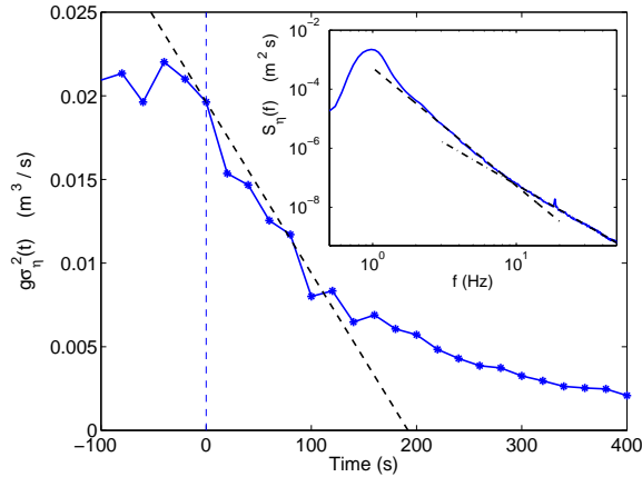
Figure 15: Temporal evolution of the gravity wave energy per unit surface and density. The wavemaker is stopped at t = 0 . Dashed line: tangent at t = 0 of slope \epsilon = 1 \times 10^{-4} (\text{m/s})^3 - see Eq. (7.7). Each value of \sigma_\eta is averaged over 20 s and averaged over 19 runs to have a good statistical convergence. Same initial forcing conditions as in figure 10. Closed basin. Inset: Wave power spectrum in the stationary regime for the same forcing conditions. Dashed line: Theoretical weak turbulence spectrum C\epsilon^{1/3}g\omega^{-4} for gravity waves with C = 1.8 and \epsilon = 1 \times 10^{-4} (\text{m/s})^3 . Dot-dashed line: f^{-17/6} power-law fit. Closed basin.
