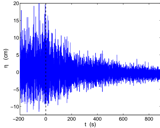
Figure 10: Decay of wave amplitude \eta(t) as a function of time for the reflecting boundary condition. Forcing is working for t < 0 and is stopped at t = 0 . Initial forcing conditions: FRN forcing with a narrow bandwidth ( f_m = 1.15 Hz, \Delta f = 0.3 Hz, \sigma_\eta = 4.6 cm).
