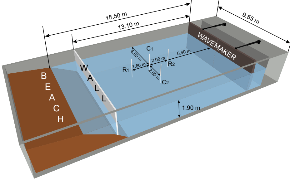
Figure 1: Sketch of the wave basin. The wavemaker is located . The boundary oppos the wavemaker is either a beach or a removable wall. The location of the array of probes is visible: capacitive probes C_1 and C_2 , and resistive ones R_1 and R_2 .
