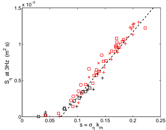
Figure 3: Amplitude of the wave spectrum amplitude S_\eta(f) measured at f = 3 Hz as a function of mean wave steepness s . Dashed line has slope 1. Forcing parameters: broad bandwidth ( f_m = 1 Hz, \Delta f = 0.6 Hz) for FRN ( \square ) or JON ( \circ ) forcings; narrow bandwidth ( f_m = 1 Hz, \Delta f = 0.3 Hz) for FRN ( + ) or JON ( \times ) forcings. Black: beach. Red (light-grey): Wall.
